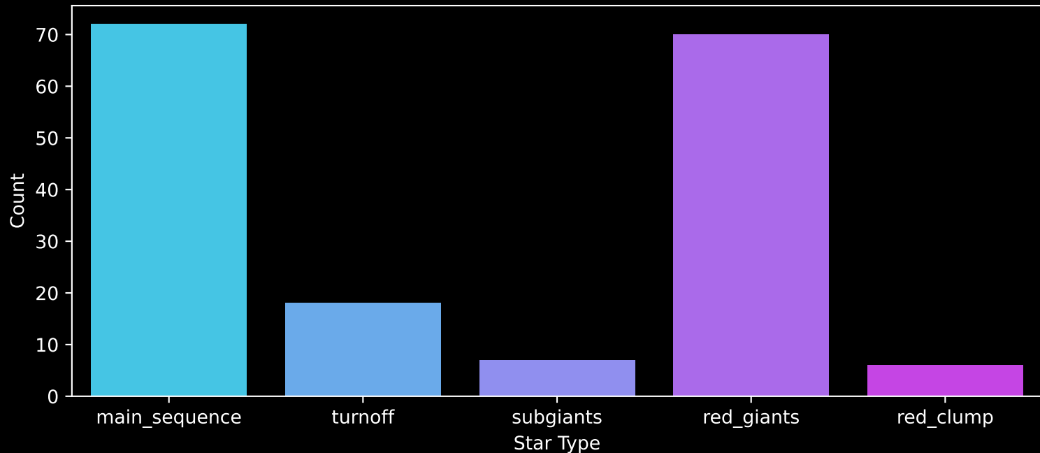
APOGEE DR17 Field: [290+60] Count plot of Star Type
