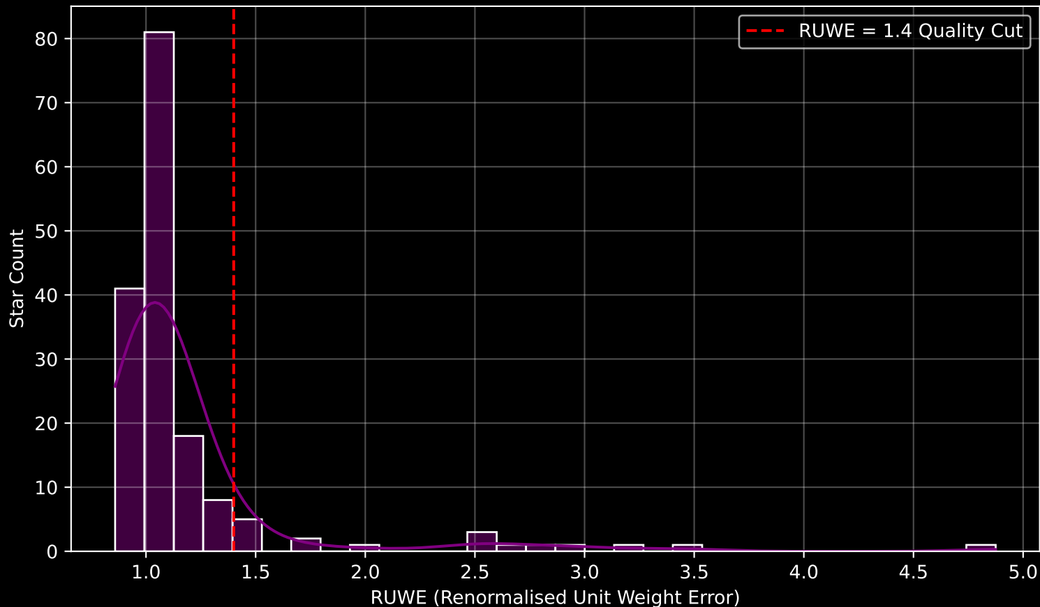
GAPOGEE DR17 Field [290+60] RUWE Distribution (n= 165)
