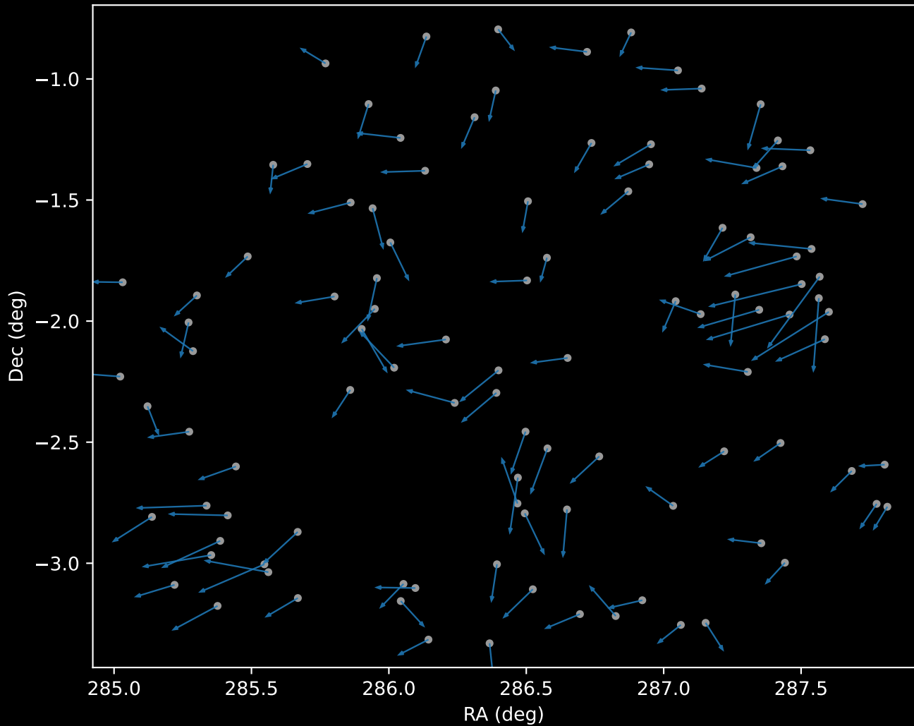
APOGEE DR17 Cluster 0 Proper Motion Vectors (n=104)
