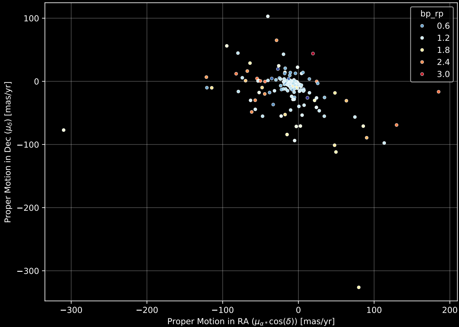
APOGEE DR17 Field: [290+60] Proper Motion Diagram (n= 173)
