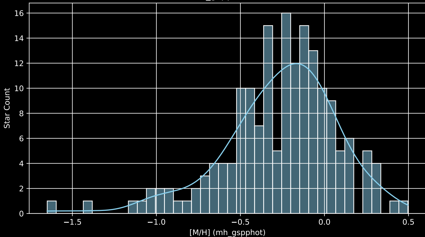
APOGEE DR17 Field: [290+60 [M/H] (mh_gspphot) (n= 173)
