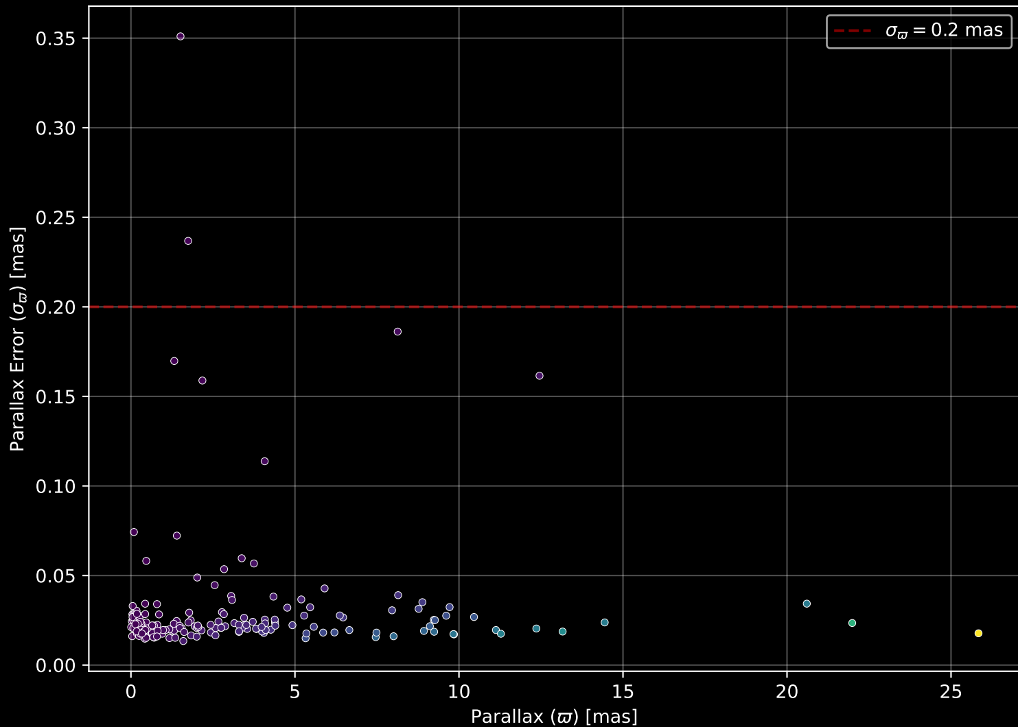
APOGEE DR17 Field: [290+60] Parallax Quality (n= 173)
